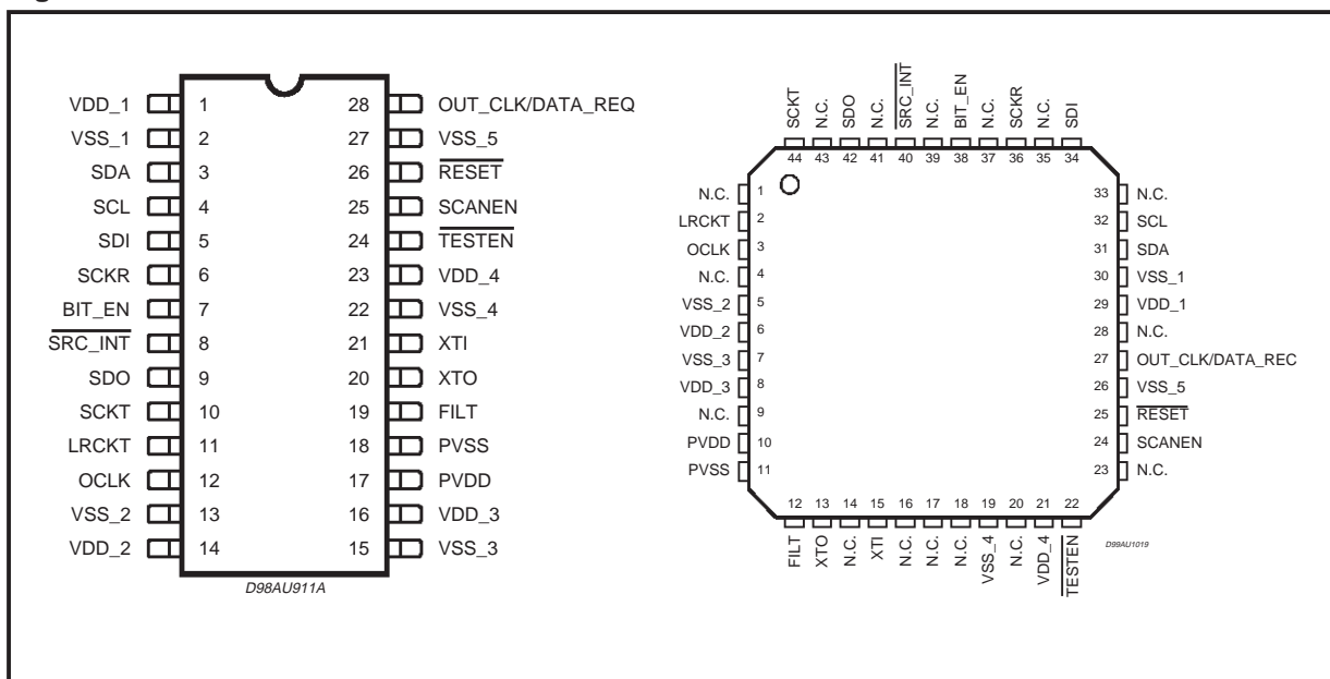
Figure 2. PIN CONNECTION
